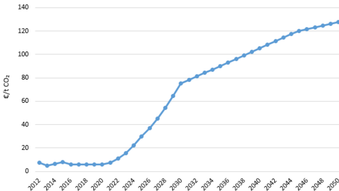
Figure 6: Assumed CO 2 price development in all scenarios [22]
