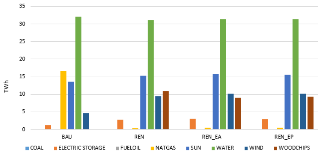
Figure 22: Electricity generation by fuel in 2030
