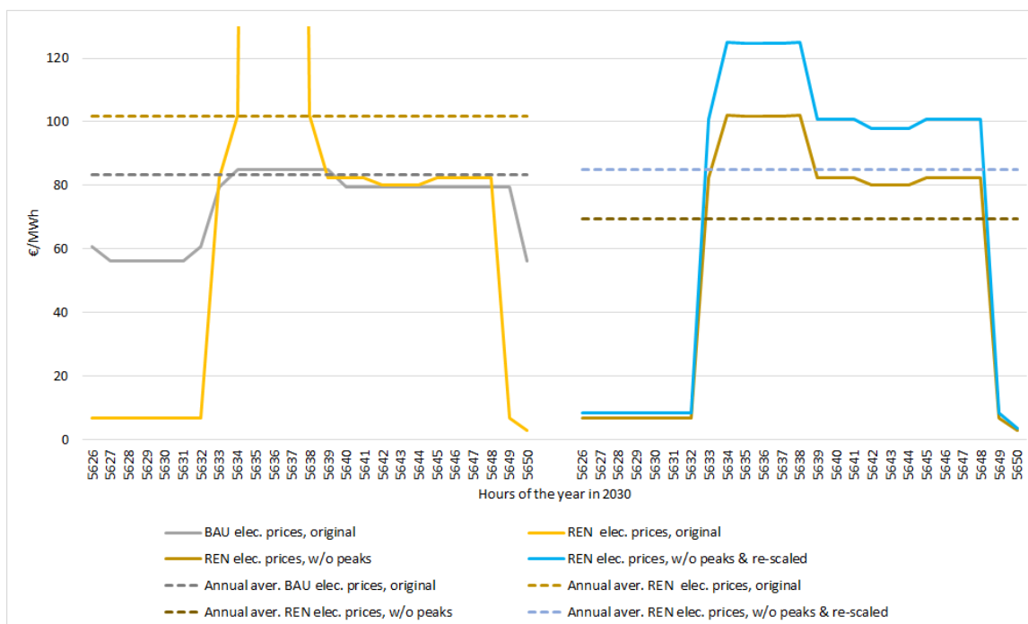
Figure 4: Example of electricity price profiles adjustments in 2030
