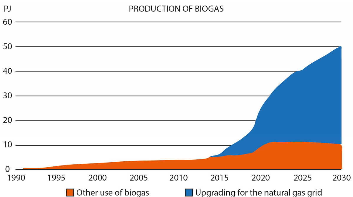
Figure 3: Development of biogas production capacity in Denmark until 2020 + Frozen policy projections 7 towards 2030. Adapted from the publication “Klimastatus og –fremskrivning 2021” by the Danish Energy Authority [6]
