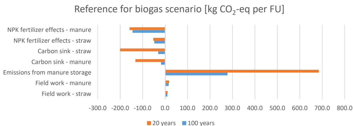
Figure 13: Climate Footprint hotspot analysis of the reference system for the biogas scenario in a 20 year and 100 year time horizon. A table with numerical results can be found in Appendix 4.
