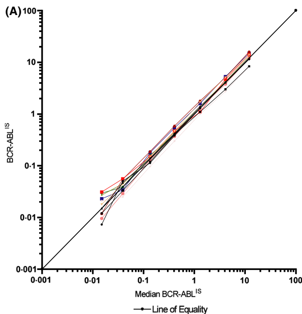
Fig 4. Linear regression for participants who performed both reverse transcriptase droplet digital polymerase chain reaction (RTddPCR) (A) and reverse transcription quantitative polymerase chain reaction (RTqPCR) (B) for samples A–G. Coloured lines represent individual participant’s results. [Colour figure can be viewed at wileyonlinelibrary.com]
