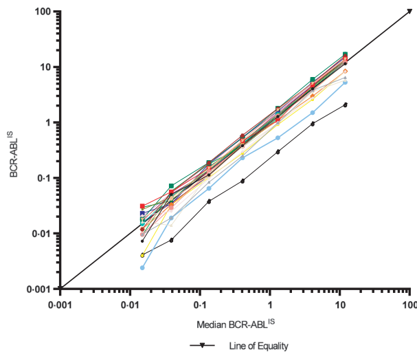
Fig 3. Linear regression for all participants who performed reverse transcriptase droplet digital polymerase chain reaction (RTddPCR) for samples A–G. Coloured lines represent individual participant’s results. [Colour figure can be viewed at wileyonlinelibrary.com]
