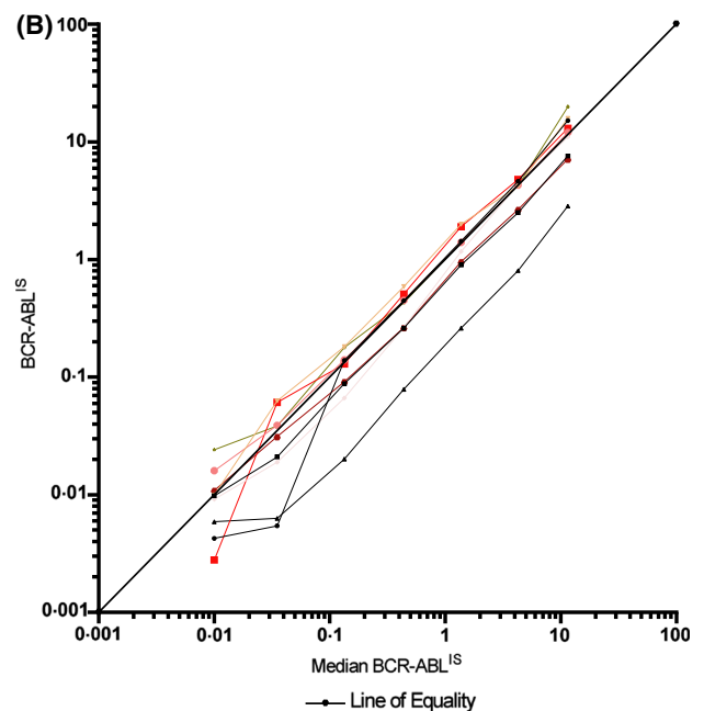
Fig 4. Linear regression for participants who performed both reverse transcriptase droplet digital polymerase chain reaction (RTddPCR) (A) and reverse transcription quantitative polymerase chain reaction (RTqPCR) (B) for samples A–G. Coloured lines represent individual participant’s results. [Colour figure can be viewed at wileyonlinelibrary.com]
