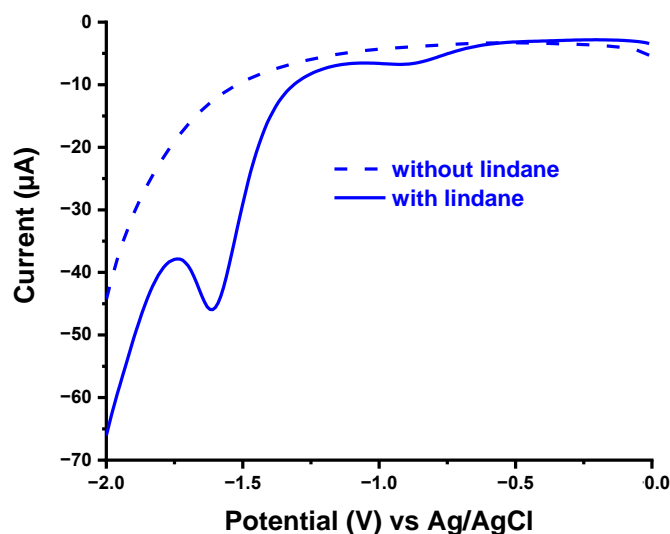
Figure 3. Square wave voltammogram in the absence (broken) and presence (solid) of lindane in nitrogen saturated 0.2 M KCl solution at glassy carbon electrode. SWV conditions: E_{\text{step}} = 0.01 V; Amplitude = 0.1 V; Frequency = 15.0 Hz.
