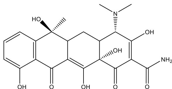
Figure 16. Tetracycline.
