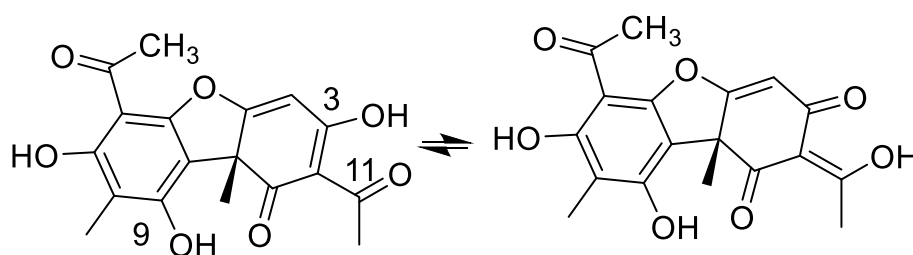
Figure 6. Tautomeric equilibrium of \beta -triketone type, usnic acid.
