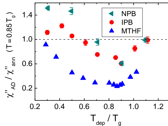
Fig. 5. Loss ratio, \chi''_{AD}/\chi''_{ann} , of MTHF, IPB, and NPB plotted against reduced deposition temperature, T_{dep}/T_g . The ratio was determined for a temperature of T = 0.85T_g based on data of Fig. 2.
