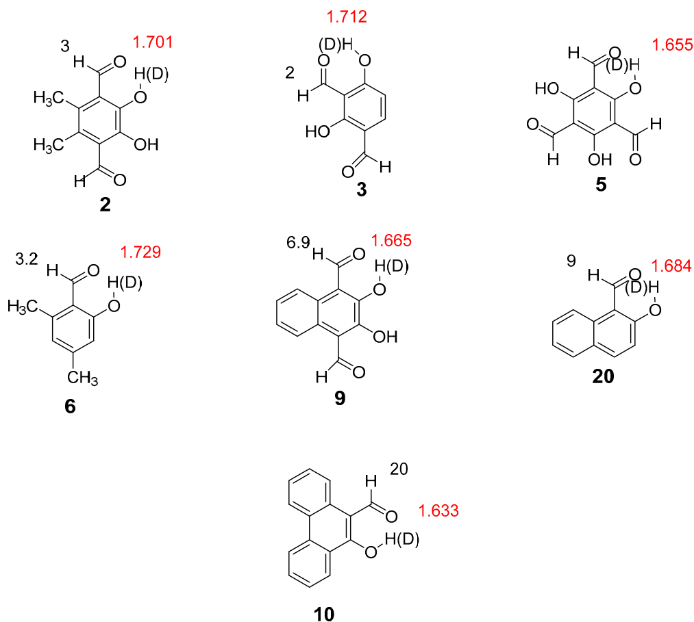
Figure 5. Experimental deuterium isotope effects on aldehyde proton ^1\text{H} -NMR chemical shifts (ppb, in black) and OH...O=C calculated distances ( \text{\AA} , in red).
