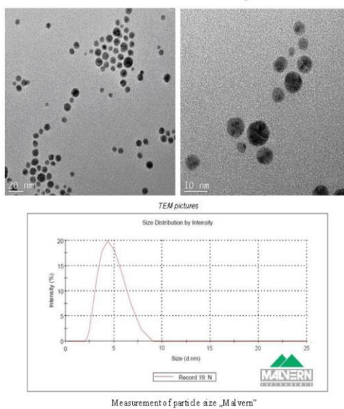
Figure S1: TEM images and size distribution from supplier (Ampox)
