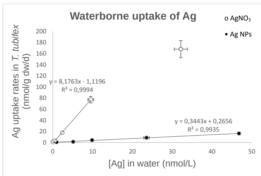
Figure 1: Silver uptake rates in T. tubifex exposure to aqueous Ag added as AgNO 3 (open circles, \pm SD) or Ag NPs (closed circles, \pm SD). The SDs are generally very low and, therefore, not all are visible.
