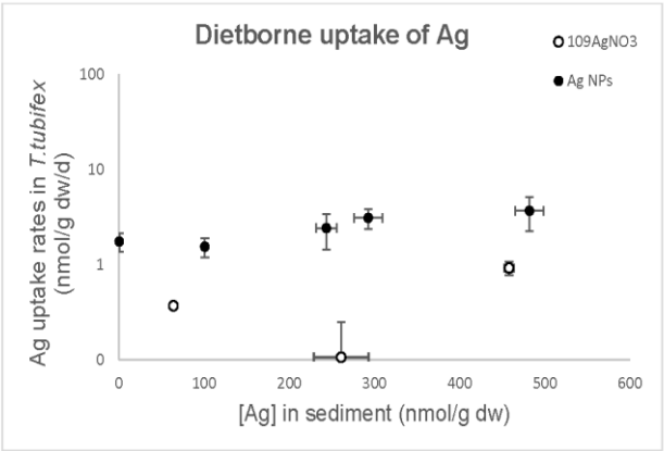
Figure S7: Dietborne uptake rates for 109 Ag (open circles, \pm SD) and Ag NPs (closed circles, \pm SD). Ag uptake rates (y-axis) are presented on logarithmic scale. Measured Ag concentrations in sediment are shown on the x-axis.
