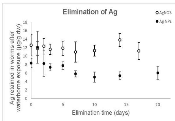
Figure S8: Elimination of Ag after 48h waterborne exposure to 3\pm 1 nmol/L AgNO 3 (open circles, \pm SD) or 58\pm 1 nmol/L Ag NPs (closed circles, \pm SD) expressed as worm body burden over time
