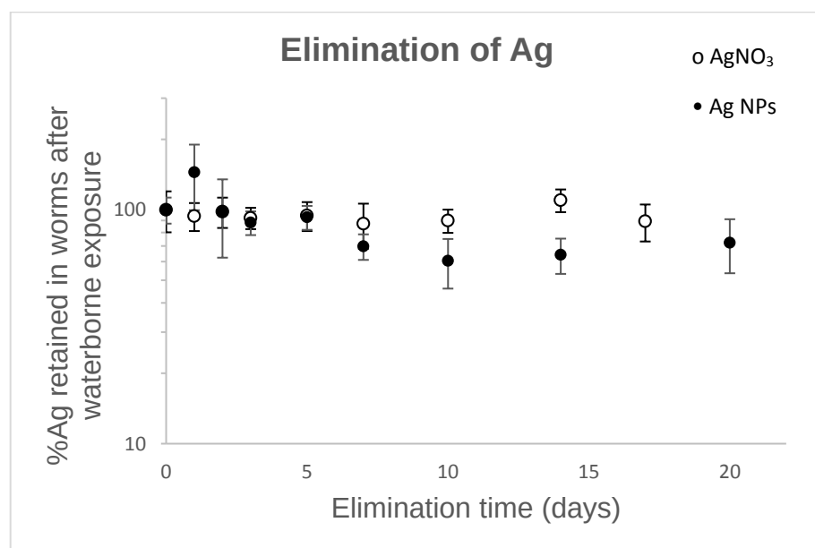
Figure 3: Ag elimination following 48h waterborne exposure to 3 \pm 1 nmol/L AgNO_3 (open circles, \pm SD ) or 58 \pm 1 nmol/L Ag NPs (closed circles, \pm SD ) expressed as % retained Ag in worm tissue over time. % Ag retained in worms (y-axis data) is shown on logarithmic scale.
