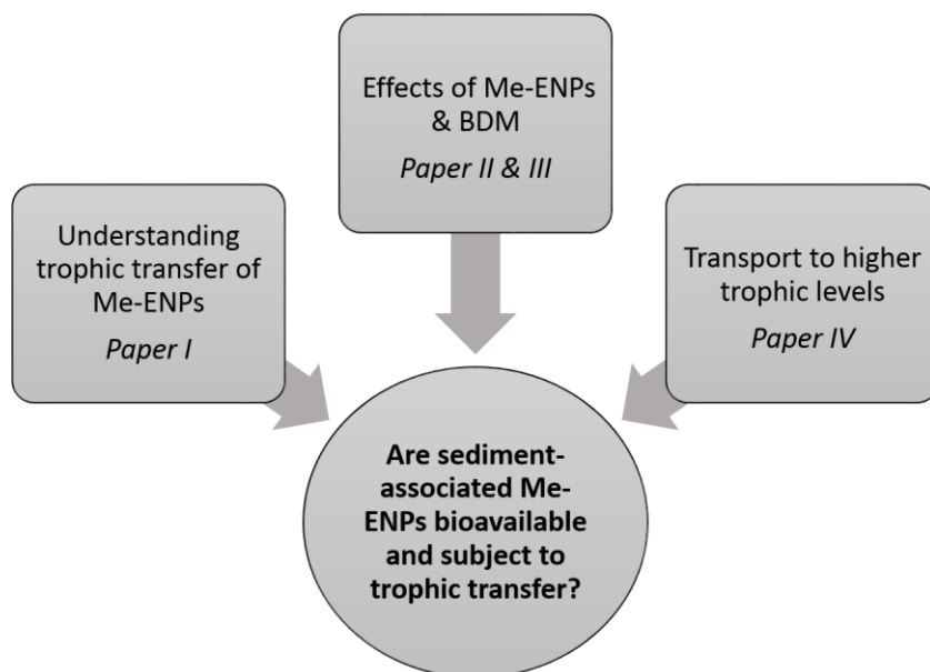
Figure 1: Schematic representation of the framework used in this thesis, displaying the 3 subtopics that support the main question of this thesis, in increasing complexity (from left to right), as well as the papers associated with each. BDM: Biodynamic modelling; Me-ENPs: Metal-based engineered nanoparticles
