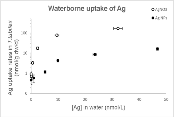
Figure S6: Waterborne uptake rates for Ag after AgNO 3 (open circles, \pm SD) and Ag NP (closed circles, \pm SD) exposure. Ag uptake rates (y-axis) are presented on logarithmic scale. Measured Ag concentrations in water are shown on the x-axis.
