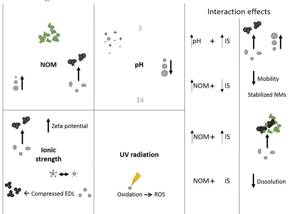
Figure 9: Schematic representation of how the four key natural parameters influencing bioavailability (NOM, pH, Ionic Strength (IS) and UV-radiation) interacts and affects Me-ENPs in the aquatic environment. Light grey represents single particles; dark grey indicates aggregated/agglomerated particles; green represents NOM; arrows indicates direction of processes (i.e. increased or decreased; smaller or larger particle sizes; leads to). EDL = electric double layer; ROS = reactive oxygen species; NMs = nanomaterials.
