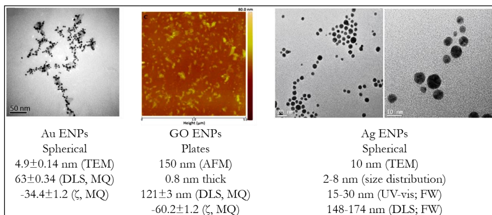
Figure 6: Overview of the Me-ENPs used in the thesis (i.e., Paper II-IV). TEM: Transmission Electron Microscopy; DLS: Dynamic Light Scattering; \zeta : Zeta-potential; MQ: MilliQ-water; AFM: Atomic Force Microscopy; FW: artificial freshwater
