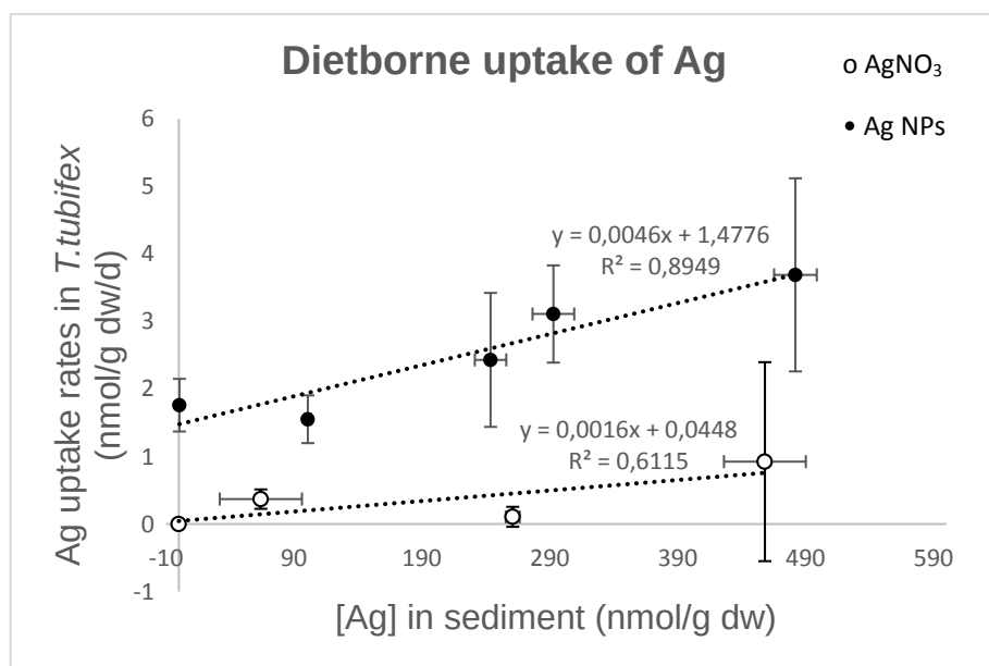
Figure 2: Dietborne uptake rates for ^{109}\text{Ag} (open circles, \pm\text{SD} ) and Ag NPs (closed circles, \pm\text{SD} ) in T. tubifex .
