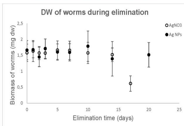
Figure S9: Biomass of worms during elimination after waterborne exposure to AgNO 3 (open circles, \pm SD) and Ag NPs (closed circles, \pm SD)
