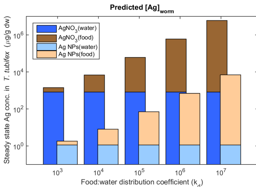
Figure 4: Model predictions using the biodynamic parameters presented in Table 2, eq.2, and k_d -values ( 10^3 to 10^7 ). [Ag]_{water} = 0.1 \mu\text{g/L} , [Ag]_{diet} was derived via use of the environmentally relevant k_d -values (i.e. around the natural k_d for Ag, 10^5 (Luoma and Rainbow, 2008)). k_d(\text{AgNO}_3) was set at 0.001 \text{ d}^{-1} . Blue is for waterborne uptake; brown is for dietborne uptake; dark colors represent the contribution of each uptake route for \text{AgNO}_3 , while the lighter colors represent the contribution of each uptake route for Ag NPs.
