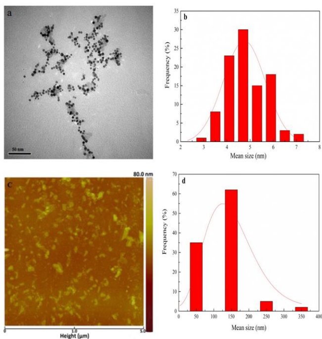
Fig. 1 – Transmission electron microscopy (TEM), atomic force microscopy (AFM) and size distribution of Au-NPs and GO-NPs in MilliQ water: (a) TEM images of 5 nm Au-NPs, (b) size distribution of Au-NPs, (c) AFM images of GO-NPs, (d) size distribution of GO-NPs. Au: gold; NPs: nanoparticles; GO: graphene oxide.
