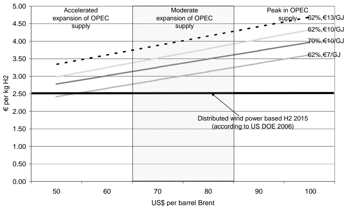
Figure 6. Hydrogen Cost at Pump for Distributed Wind Power based Electrolysis and Natural Gas based Reforming with varying Performance Parameter Values.
