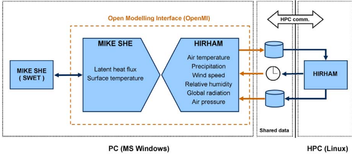
Figure 4. Schematic of the HIRHAM-MIKE SHE coupling. Both model codes have been extended with OpenMI Linkable Components, exposing selected variables to each other within the OpenMI platform. The MIKE SHE code runs on the same PC (MS Windows) as the OpenMI software, whereas the HIRHAM code runs on a massively parallelized Cray XT5 high performance computer system (HPC). Linking directly to the HPC is not possible, necessitating data exchange by files and introducing a considerable overhead in simulations. Figure from Butts et al. (2014).
