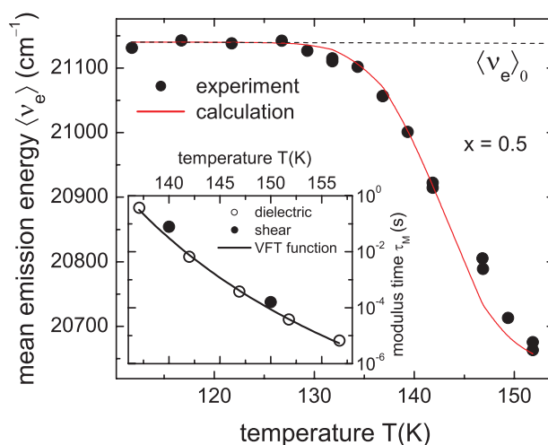
FIG. 9. The dots represent the temperature dependence of the average emission energy \langle\nu_e\rangle (in units of \text{cm}^{-1} ) of 10^{-4} mol QX in (2\text{E1H})_{0.5}(\text{2E1Br})_{0.5} recorded 10 ms after laser excitation. The dashed line marks the low-temperature plateau \langle\nu_e\rangle_0 . The solid line is calculated from Eq. (6) using the modulus time scale \tau_M represented in the inset as solid line and with the parameters given in the text. The plot in the inset also shows the times from the dielectric and from the shear modulus.
