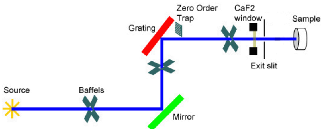
Figure 1.16: Schematic of the CD1 beamline on the ASTRID storage ring. The monochromator is operated at beamline vacuum and separated from sample compartment by a \text{CaF}_2 window. This figure is taken from http://www.isa.au.dk/facilities/astrid/beamlines/cd1/CD1OpticalSpecs.asp (June 24 th , 2010) with a slight modification. The PEM (Photo Elastic Modulator) component which is placed before sample holder and used to convert linearly polarized light to circularly polarized light in synchrotron radiation circular dichroism (SRCD) spectroscopy is removed.
