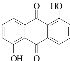
Figure 5.1: Molecular structure of Anthrarufin
