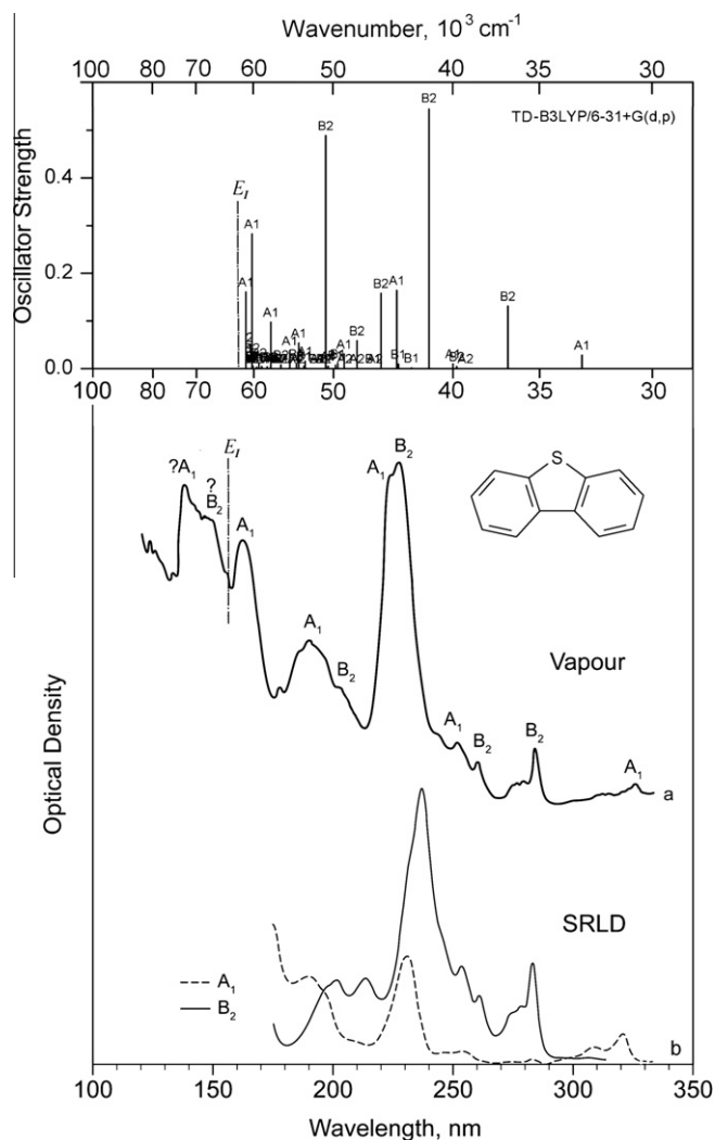
Fig. 4. Electronic spectra of dibenzothiophene: (top) Theoretical. (bottom) Experimental: (a) gas phase spectrum and (b) synchrotron radiation linear dichroism spectra.
