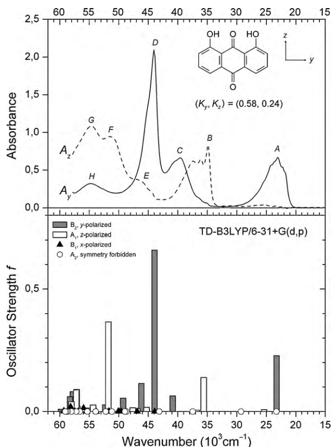
Fig. 3. Top: Partial absorbance curves A_y(\tilde{\nu}) and A_z(\tilde{\nu}) for chrysazin ( C ) aligned in stretched polyethylene, corresponding to long- and short-axis polarized absorption (full and dashed line). The LD absorbance curves were measured with synchrotron radiation, except for the region below 32,000\text{ cm}^{-1} where a conventional light source was used. Bottom: Theoretically predicted transitions (Table 2).
