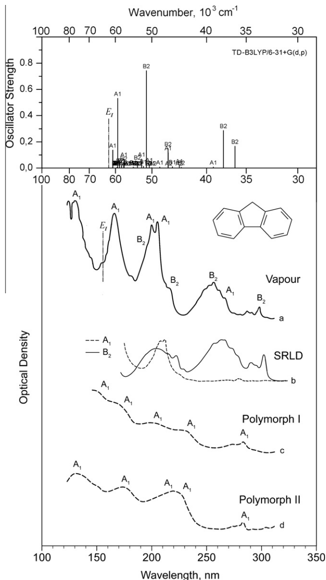
Fig. 1. Electronic spectra of fluorene: (top) Theoretical. (bottom) Experimental: (a) gas phase spectrum, (b) synchrotron radiation linear dichroism spectra, (c) polymorph I crystal spectrum, (d) polymorph II crystal spectrum, ab crystallographic plane.
