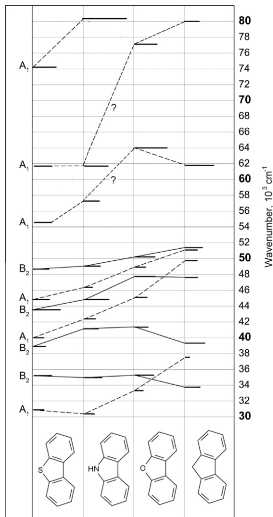
Fig. 5. Diagram of energy levels for all four compounds (in \text{cm}^{-1} ); transitions of A_1 symmetry are connected by dashed lines, those of B_2 symmetry by solid lines.
