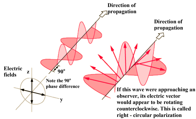
Figure 1.3: Right-Circular polarized light
