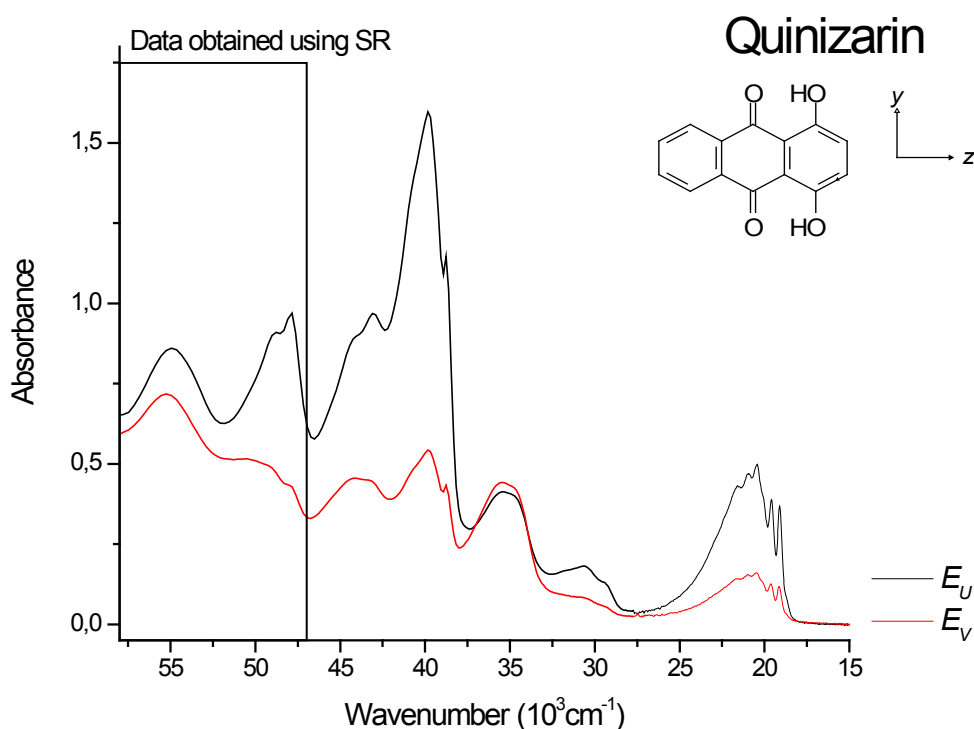
Figure 1.17: The SRLD spectra of Quinizarin with extended spectral region ca. 11000 \text{ cm}^{-1} (from 47000 \text{ cm}^{-1} to 58000 \text{ cm}^{-1} ). The sample is partially aligned in stretched LDPE. The two LD curves ( E_U - black and E_V - red solid curves) are measured at room temperature in spectral region from ca. 27000 \text{ cm}^{-1} (360 nm) to ca. 58000 \text{ cm}^{-1} (170 nm) at the CD1 beamline on the ASTRID storage ring at the Institute for Storage Ring Facilities (ISA), Aarhus University. The low energy absorption band is measured at room temperature on a traditional spectrophotometer (UV-VIS scanning spectrophotometer – UV-2101PC Shimadzu) at our laboratory, Roskilde University.
