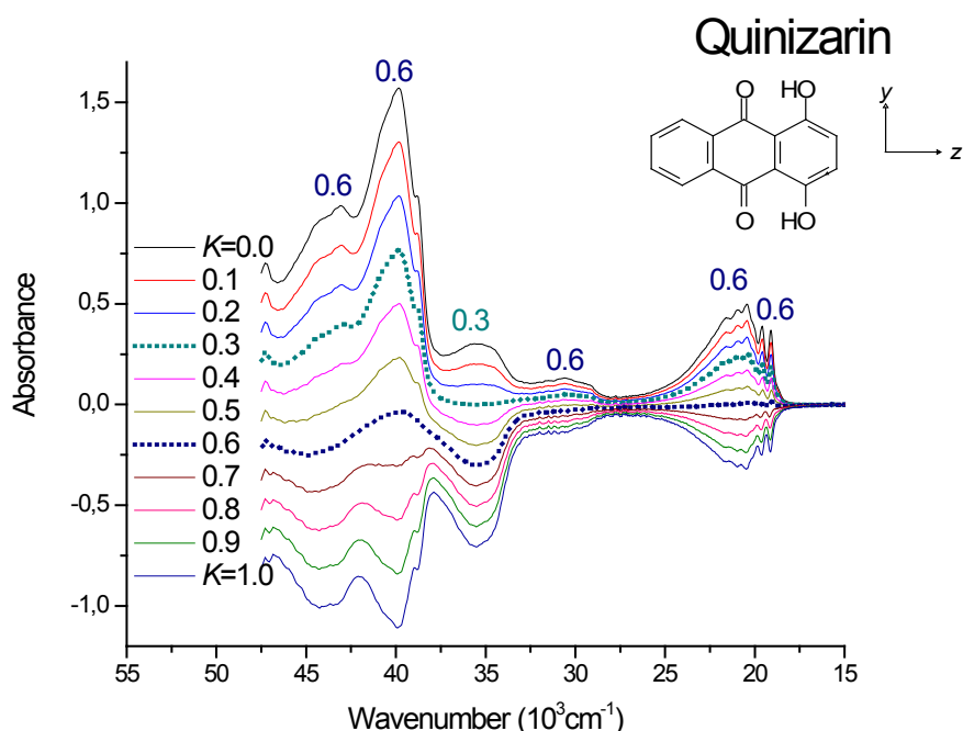
Figure 1.10: Trial-and-Error Method (TEM). The linear combination of the two independent LD curves ( E_U and E_V ) produces a family of reduced spectra. And value of orientation factor of an absorption band is visually determined as described in the text.
