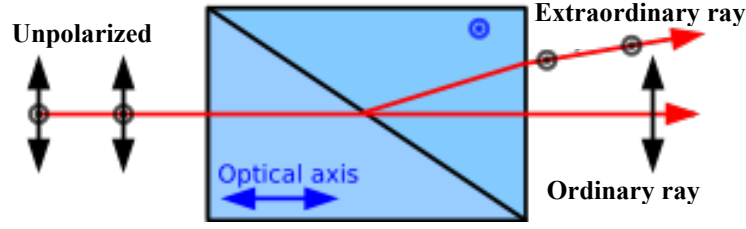
Figure 1.7: Rochon polarizer. Both ordinary ray (o-ray) and extraordinary ray (e-ray) are transmitted through, but the e-ray is deviated while the o-ray is not.
