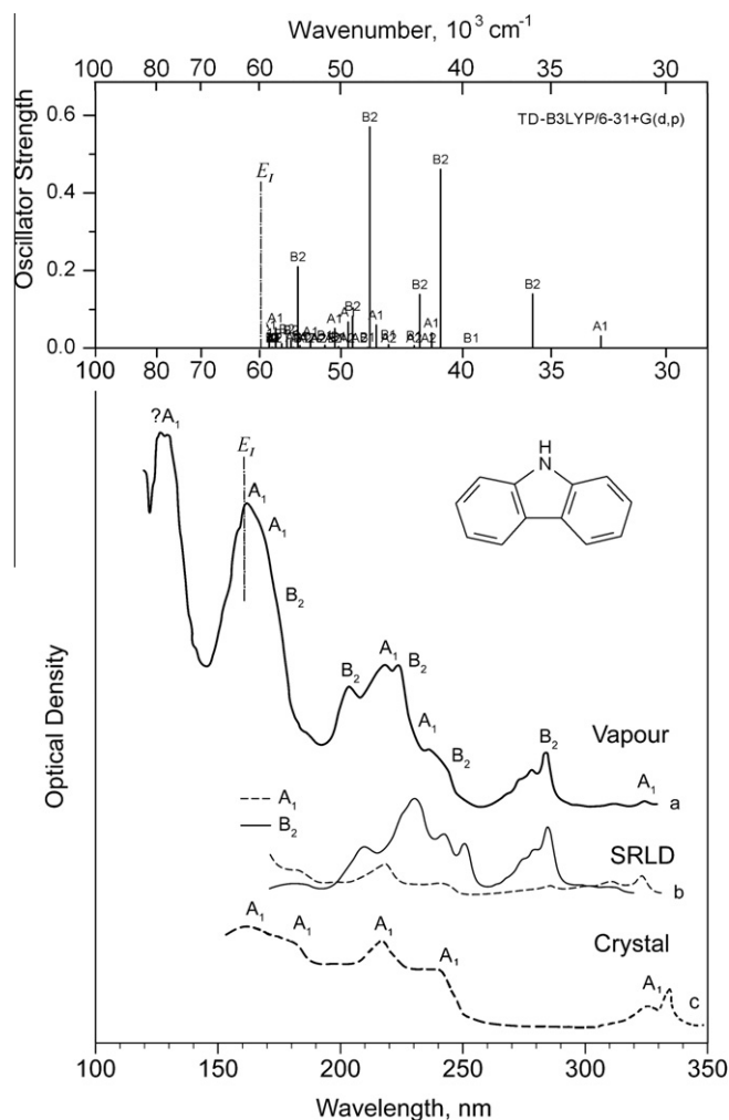
Fig. 3. Electronic spectra of carbazole: (top) Theoretical. (bottom) Experimental: (a) gas phase spectrum, (b) synchrotron radiation linear dichroism spectra, (c) crystal spectrum, ab crystallographic plane.
