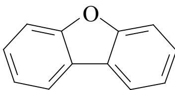
Figure 4.1: Molecular structure of dibenzofuran (DBF)
