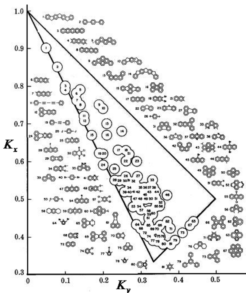
Figure 1.14: The relationship between molecular shape and experimental value of orientation factor (This figure is also taken from: J. Michl, E.W. Thulstrup, Spectroscopy with polarized light. Solute alignment by photoselection, in liquid crystals, polymers and membranes , VCH publishers, Inc., New York 1986, 1995) with slight modification on axis labels according to the convention in figure 1.12.
