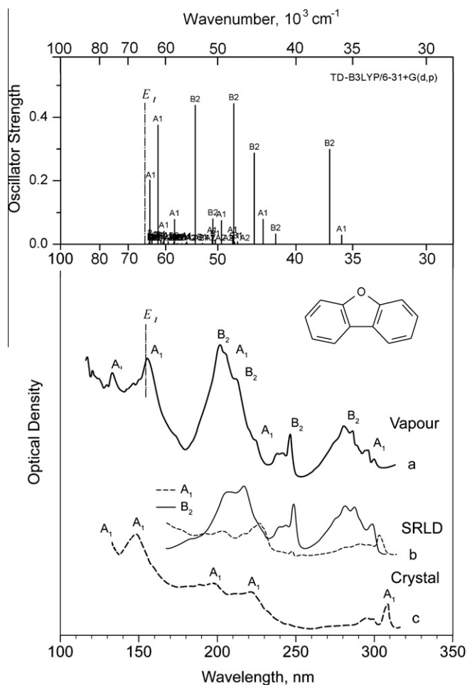
Fig. 2. Electronic spectra of dibenzofuran: (top) Theoretical. (bottom) Experimental: (a) gas phase spectrum, (b) synchrotron radiation linear dichroism spectra, (c) crystal spectrum, ab crystallographic plane.
