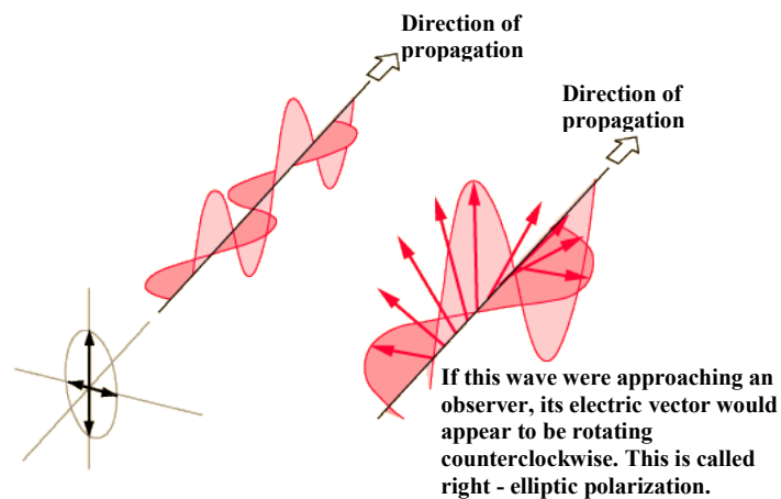
Figure 1.4: Right-Elliptical polarized light
