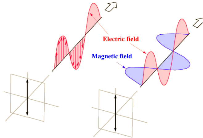
Figure 1.2: Linearly polarized light
