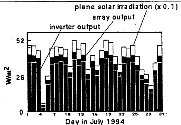
Fig. 4. July performance of Brædstrup installation [2].
