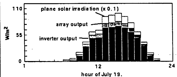
Fig. 5. Performance of Brædstrup installation on July 19, 1994. [2]
