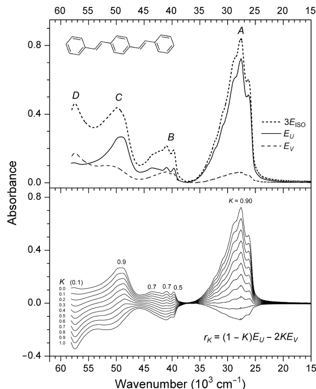
Fig. 1. Top: Linear Dichroism (LD) absorbance curves E_U(\tilde{\nu}) and E_V(\tilde{\nu}) for 1,4-distyrylbenzene (DSB) in stretched polyethylene measured at room temperature with the electric vector of the sample beam parallel and perpendicular to the uniaxial stretching direction U . 3E_{\text{ISO}}(\tilde{\nu}) = E_U(\tilde{\nu}) + 2E_V(\tilde{\nu}) is three times the absorbance that would have been measured in an isotropic experiment on the same sample. Bottom: Family of reduced absorbance curves r_K(\tilde{\nu}) = (1-K)E_U(\tilde{\nu}) - 2KE_V(\tilde{\nu}) with K varying from 0 to 1 in steps of 0.1.
