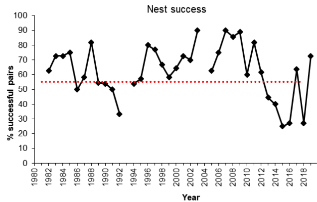
Figure 1: Nest success - proportion of occupied sites that produced young; the red line is the threshold where there “would be cause for concern in the short term” (USFWS) 9 .
