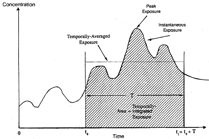
Figure 2.5 A hypothetical exposure time profile that illustrates the instantaneous point exposure, the integrated exposure, the average exposure and the peak exposure (maximum exposure) from Zartarian et al. (1997).
