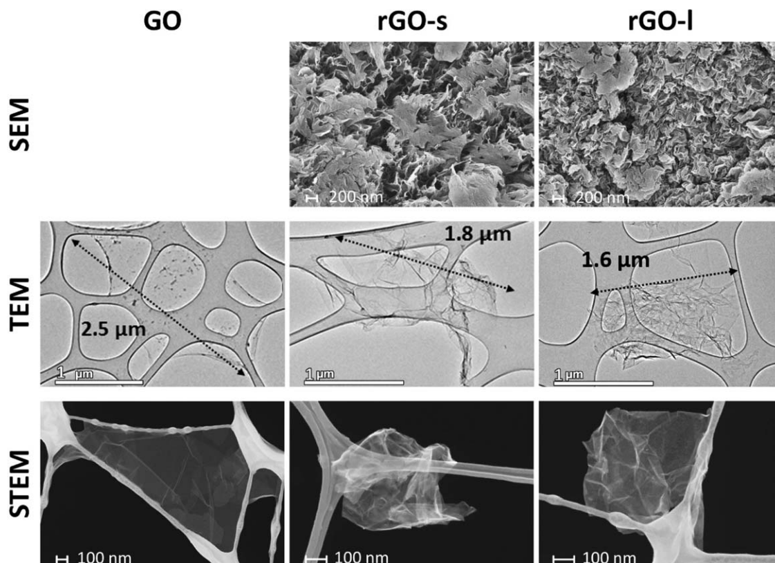
Fig. 2. Morphology of GO (Left), rGO-s (middle), and rGO-I (right): Agglomeration of graphene layers visualized by SEM microscopy. The Lateral size of graphene layers was determined by TEM and STEM microscopy.
