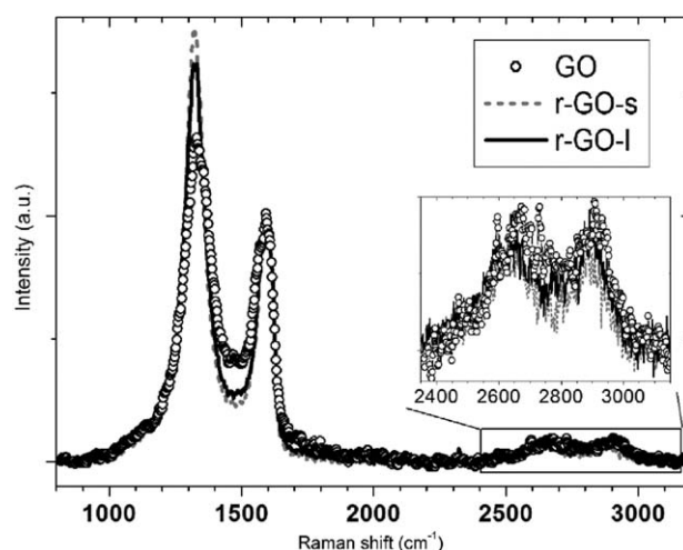
Fig. 1. 633 nm Raman spectra of isolated flakes of GO, rGO-s, and rGO-l normalized to the G peak intensity ( \sim 1,595 \text{ cm}^{-1} ).
