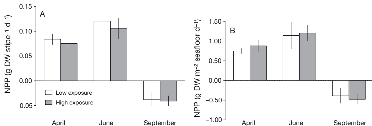
Fig. 8. Net primary production (NPP) of epiphytic macroalgae on the stipes of Laminaria hyperborea from sites with low and high wave exposure during spring, summer and fall, respectively. NPP is: (A) per stipe; and (B) per \text{m}^{-2} of seafloor. Data are means \pm 1 SD (across sites; n = 3 )
