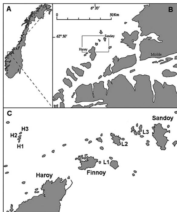
Fig. 1. (A) Norway and (B) the Molde archipelago with an indication of (C) the 6 study sites situated around and between the islands of Haroy, Finnoy and Sandoy
