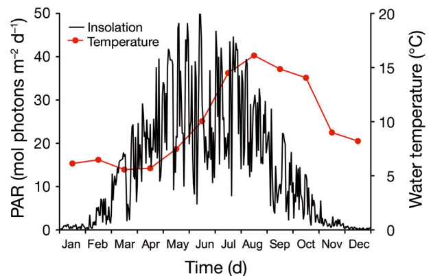
Fig. 3. Daily solar irradiance (photosynthetically active radiation, PAR) and water temperature near the study site from January to December 2006. Light data were obtained from LanbruksMeterologisk Tjeneste, site Tingvoll ( 62^{\circ} 91' \text{N} , 08^{\circ} 17' \text{E} ), while water temperatures were obtained from Institute of Marine Research ( www.imr.no/forskning/forskningsdata/stasjoner/ ), site Bud ( 62^{\circ} 54' \text{N} , 06^{\circ} 54' \text{E} )
