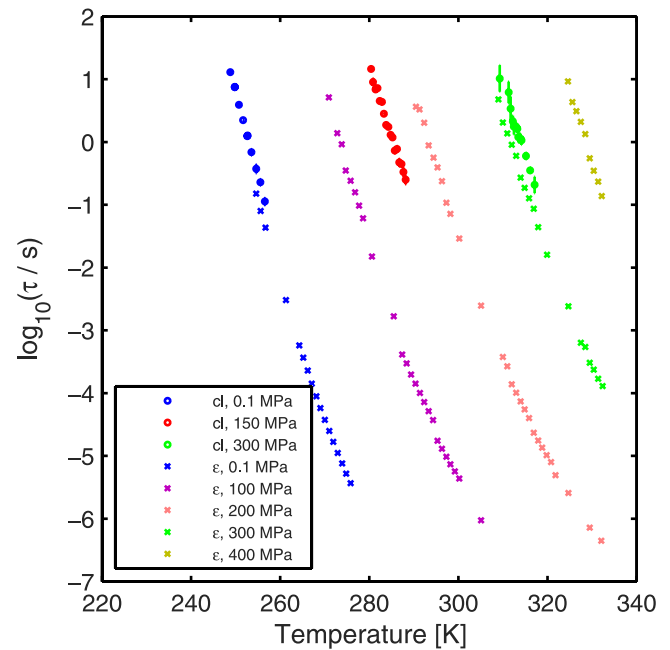
FIG. 2. Comparison of the relaxation times ( \tau ) for the specific heat measurements (same data as on Fig. 1) and the dielectric measurements at the indicated pressures.
