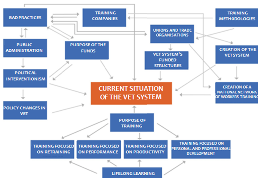
Figure 1. Conditional matrix
