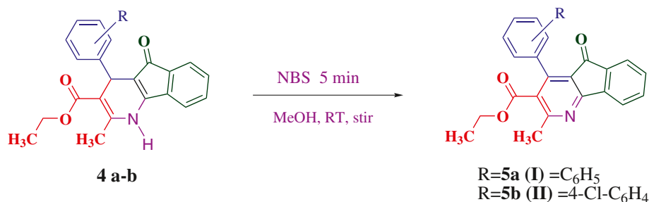
Scheme 2 Synthesis scheme of the compounds I and II.
