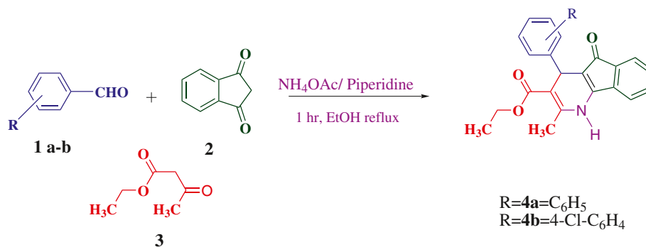
Scheme 1 Synthesis scheme of the dihydropyridines.
