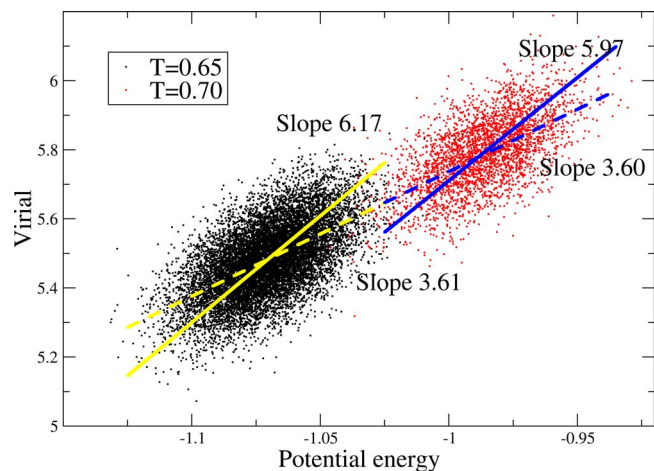
FIG. 8. (Color online) Scatter plot of W, U -correlations for the Dzugutov system at density 0.88 and temperatures 0.65 and 0.70 ( NVE ). The dashed lines indicate the best-fit line using linear regression. These are consistent with the temperature dependence of the mean values of \langle W \rangle and \langle U \rangle , as they should be (see Appendix B), but they clearly do not represent the direction of greatest variance. The full lines have slopes equal to the ratio of standard deviations of the two quantities [Eq. (7)]. The correlation coefficient is 0.585 and 0.604 for T=0.65 and T=0.70 , respectively.
