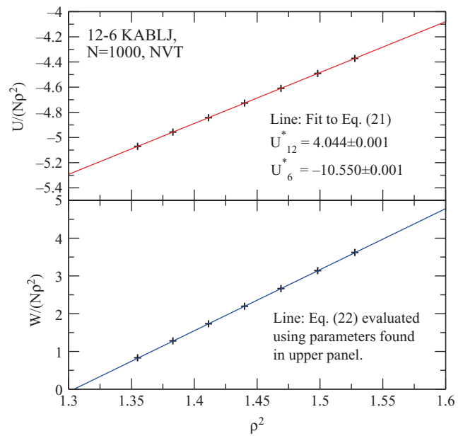
FIG. 6. Test of a 12-6 KABLJ isomorph (same as in Figs. 1 and 2). Top panel: U fitted to Eq. (21) using \rho_* = 1 (i.e., \tilde{\rho} = \rho ). Bottom panel: W compared to Eq. (22), using the parameters U_m^* and U_n^* found in the top panel.
