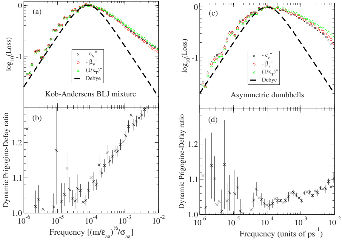
FIG. 1. (Color online) (a) shows the imaginary parts (scaled to maximum value) of -c_v(\omega) , -\beta_v(\omega) , and 1/\kappa_T(\omega) for the Kob-Andersen binary Lennard-Jones (BLJ) 80-20 mixture [27]; (c) shows the same for a system of asymmetric dumbbells [28]. The dashed lines indicate Debye relaxation with relaxation times \tau_\alpha = 2000 \sigma_{aa} \sqrt{m/\epsilon_{aa}} and \tau_\alpha = 1600 ps, respectively. (b) and (d) show the corresponding dynamic Prigogine-Defay ratios, Eq. (2). For both systems the total simulation time covers more than 10^4 \tau_\alpha .
