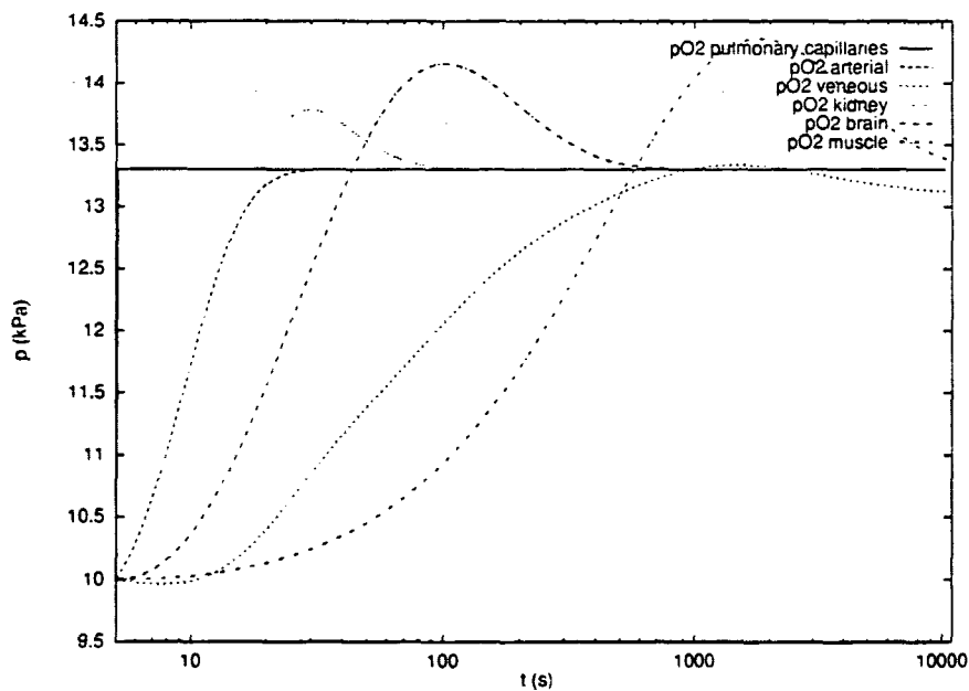
Figure 7.16: Oxygen tension in various compartments without metabolism
