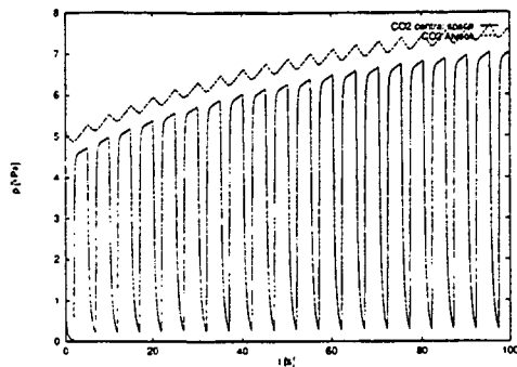
Figure 7.7: p_{\text{CO}_2} in a lung with low compliance
