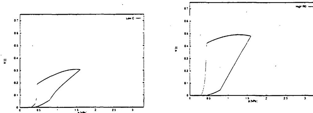
Figure 7.4: pV diagram generated with high airways resistance R_0 = 2 * R_{0, std}
